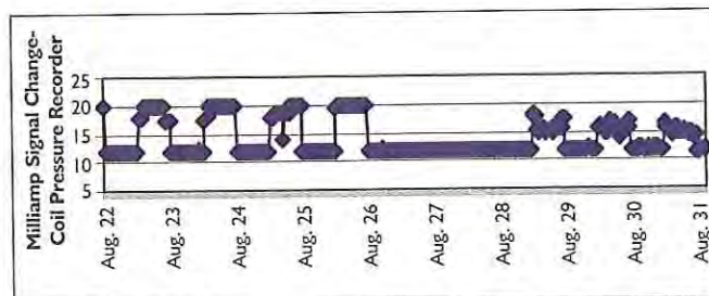
Figure 3: SF-8 differential pressure across coil change before/after cleaning.
