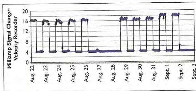
Figure 2: SF-9 air velocity increase before/after cleaning.
