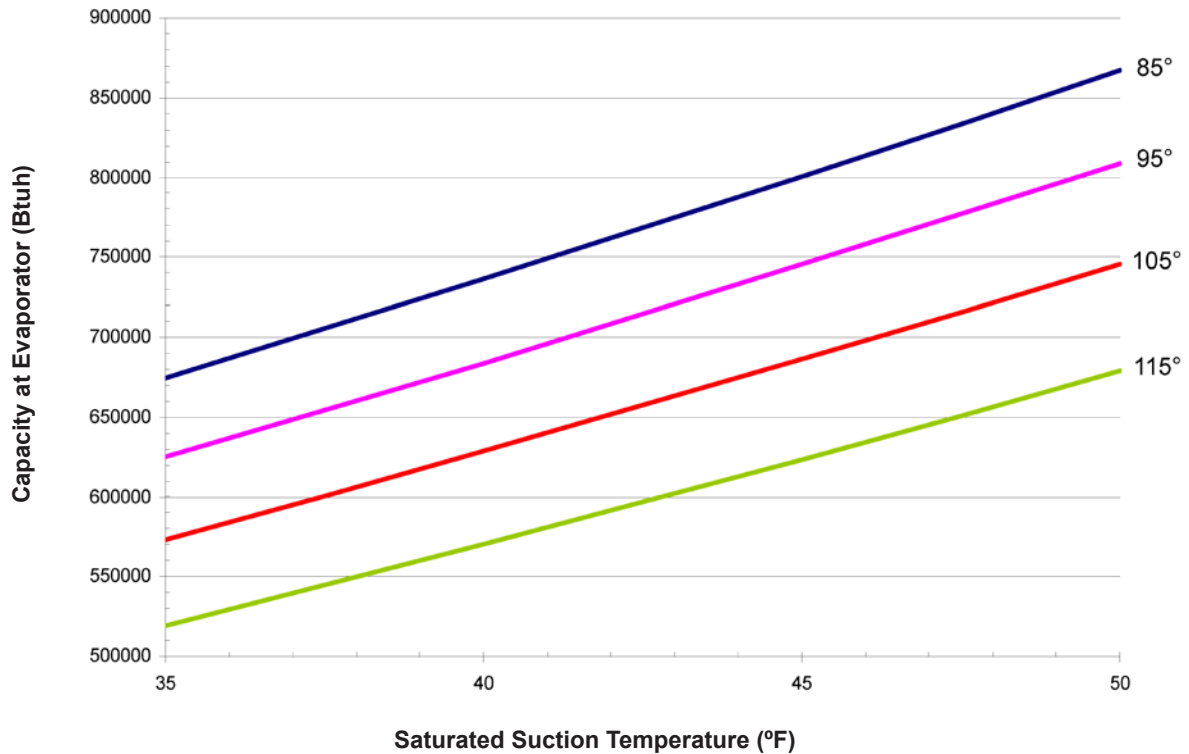
Figure 15: RCS 072D Unit Capacity Chart
