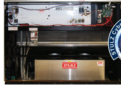
STULZ CyberMOD Installed
