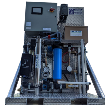
Treatment and Control Systems
